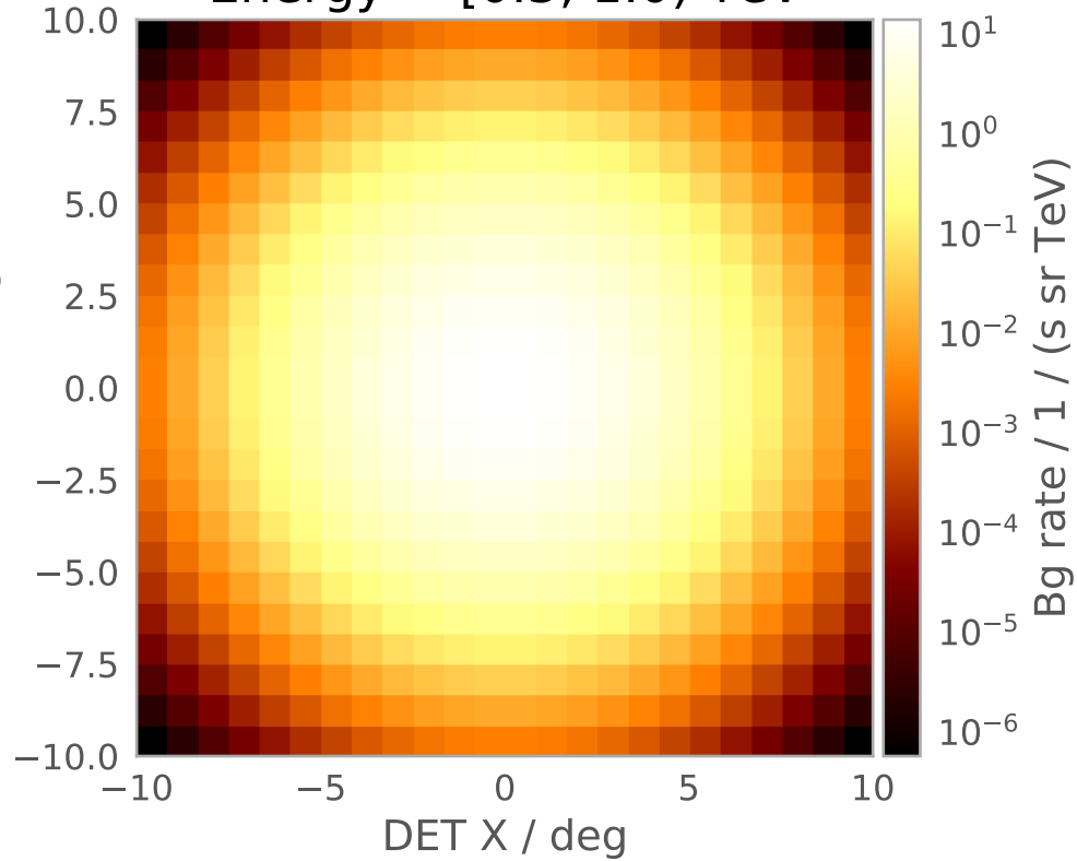
Energy = [0.3, 1.0) TeV
