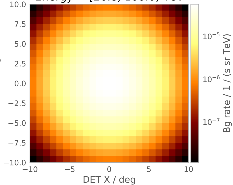
Energy = [26.8, 100.0) TeV
