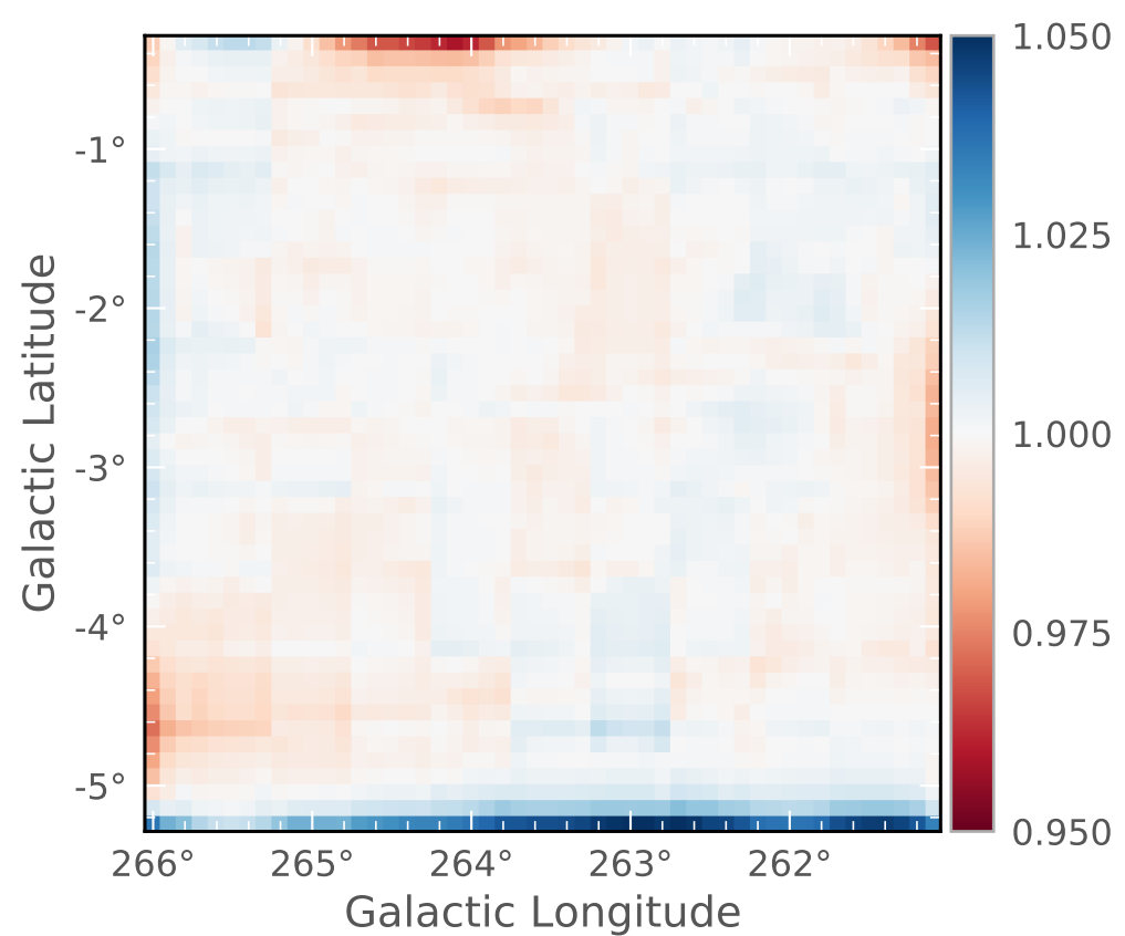
Ratio: Gammamy/Fermi Tools
