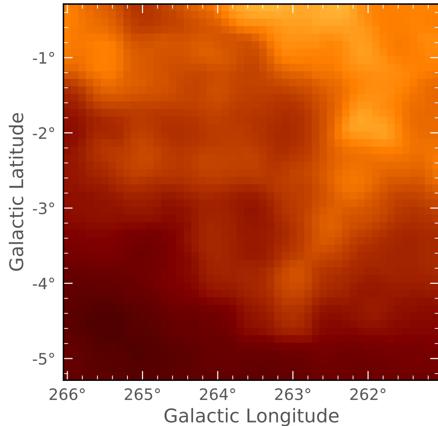
Gammamy Background
