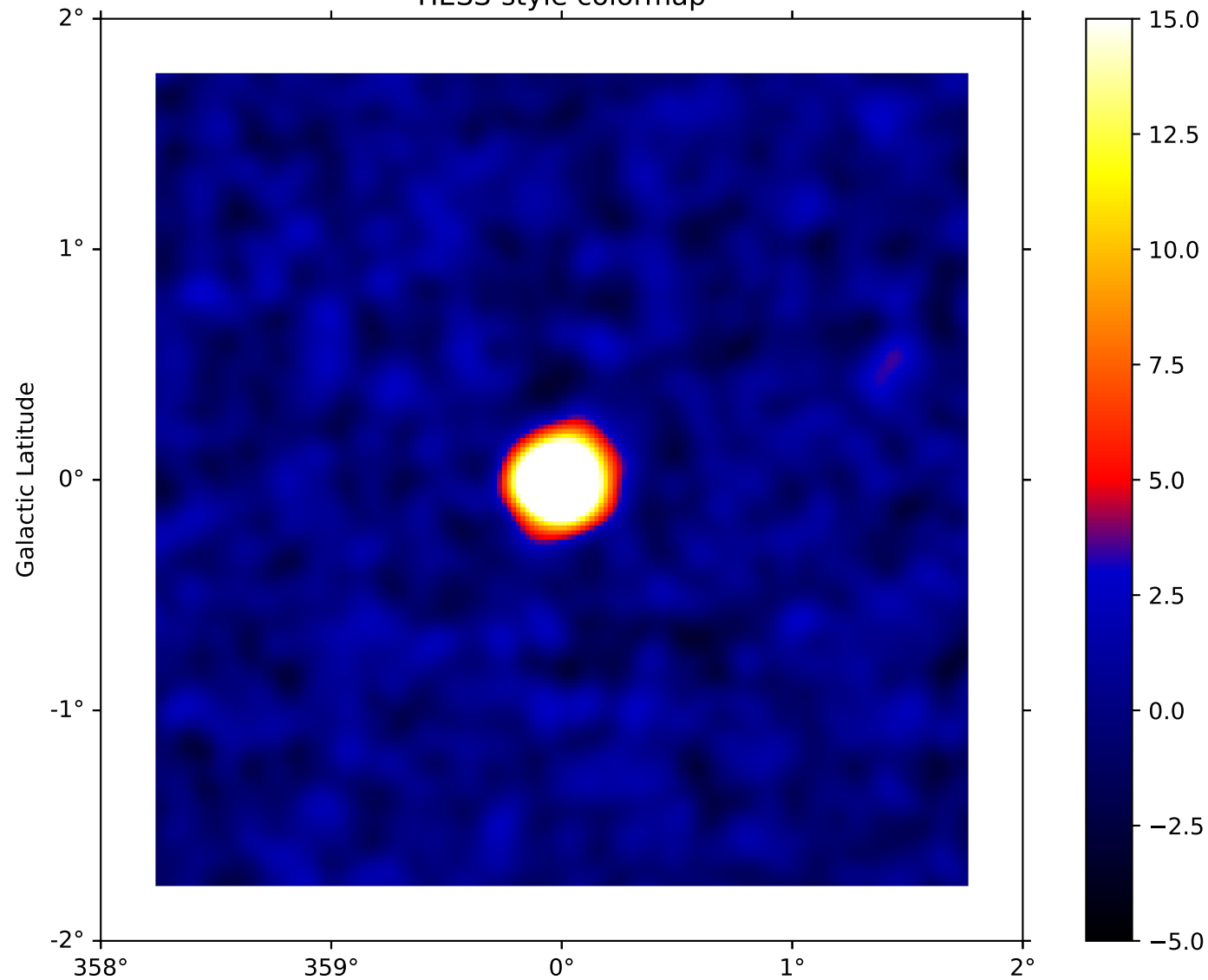
HESS-style colormap
