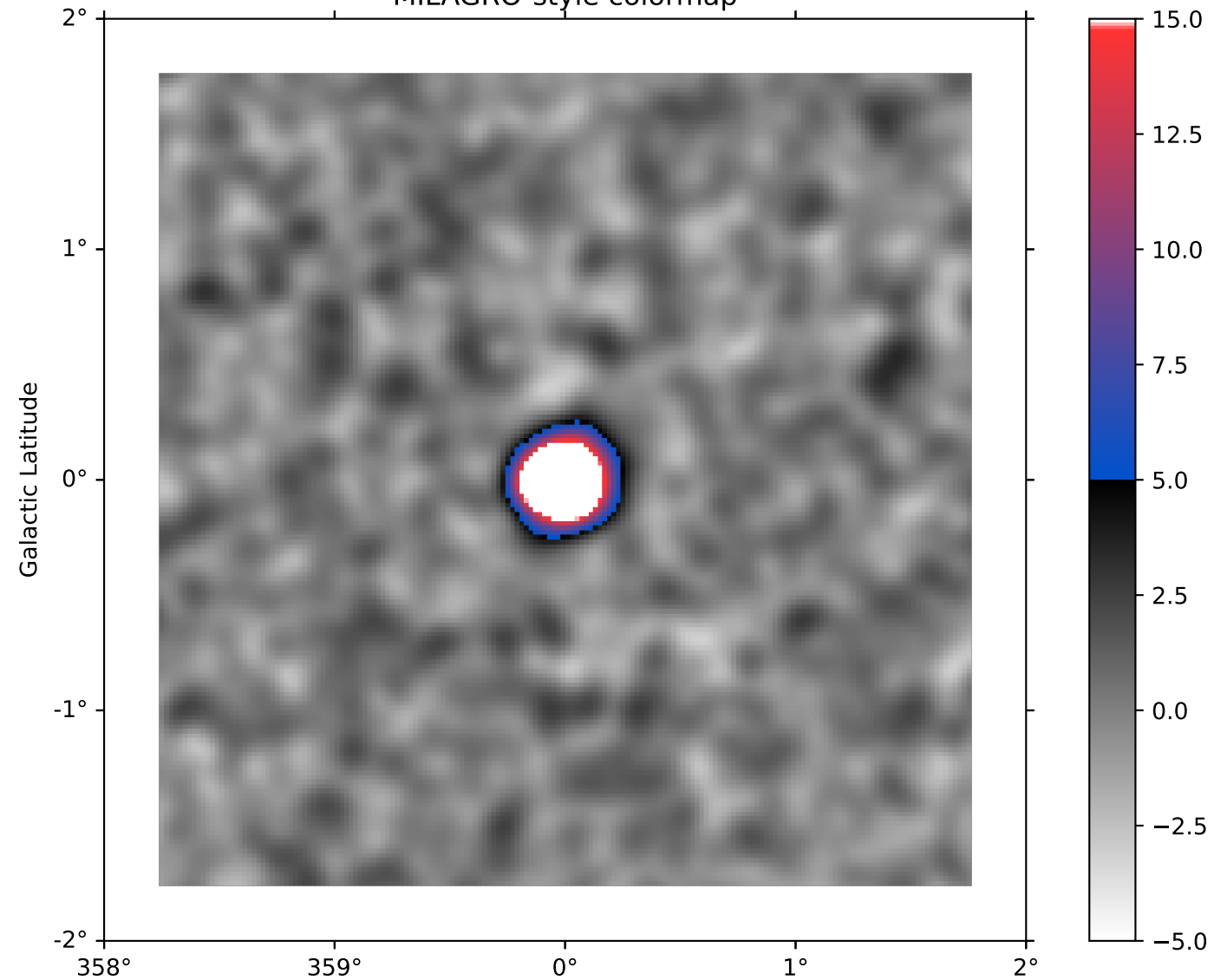
MILAGRO-style colormap
