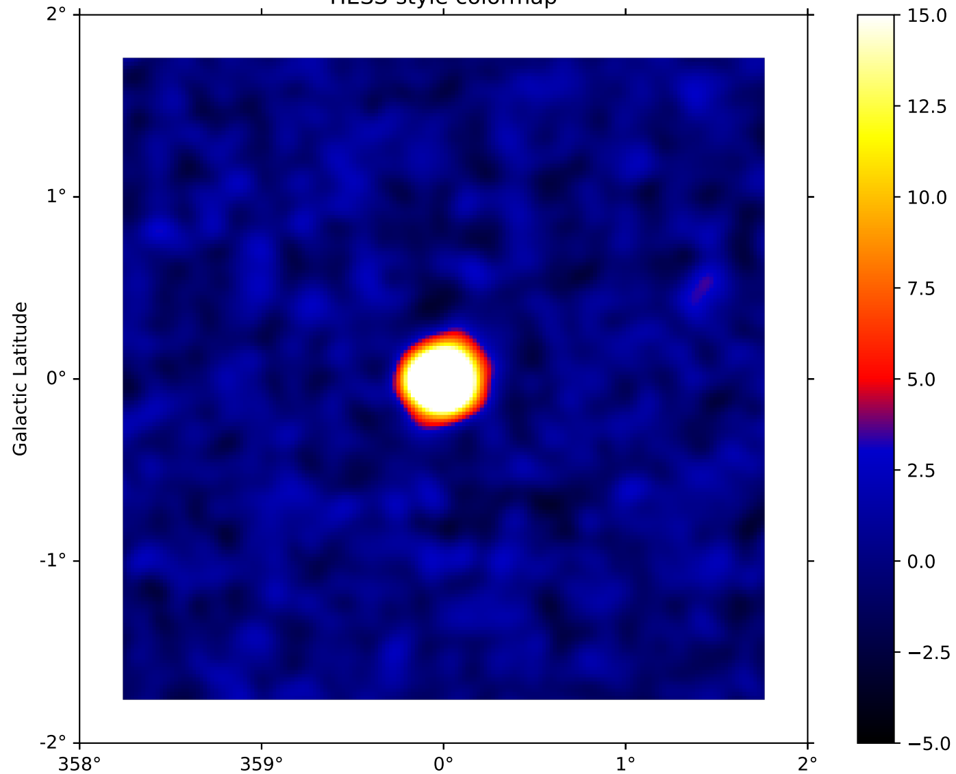
HESS-style colormap
